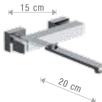
501PA POLAR Miscelatore monocomando lavello a parete bocca girevole. Wall mtg. single-lever sink mixer with swivel spout.
