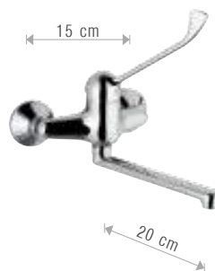
580E9 EPIC Miscelatore monocomando lavello a parete bocca girevole con leva clinica. Wall mtg. single-lever sink mixer with swivel spout and clinic lever.
