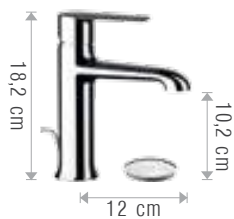
393AR Miscelatore monocomando lavabo con scarico. Single-lever basin mixer with pop-up waste. CR FIN ( .14 .08 )
