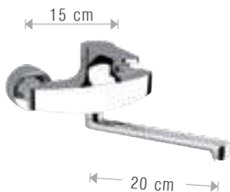
501SF SURF Miscelatore monocomando lavello a parete canna girevole. Wall mtg. single-lever sink mixer with swivel spout.
